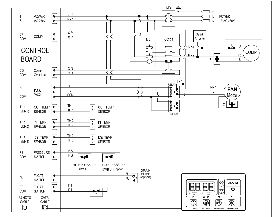
Figure 38 - Circuit Wiring Diagram (Models WPC-7000 / WPC-9000 )
