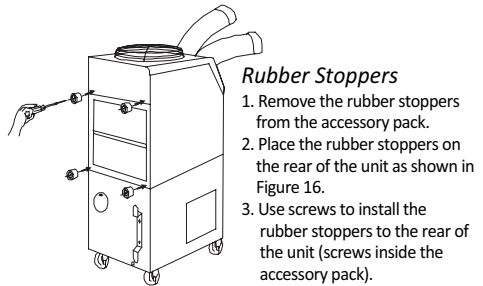
Figure 16 – Rubber Stopper attachment
