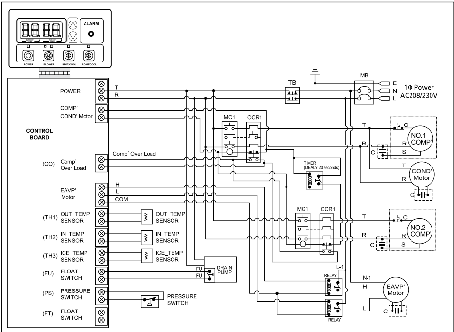
Figure 39 - Circuit Wiring Diagram (Models WPC-15000 )
