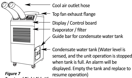
Figure 7 Front and Right Side View
