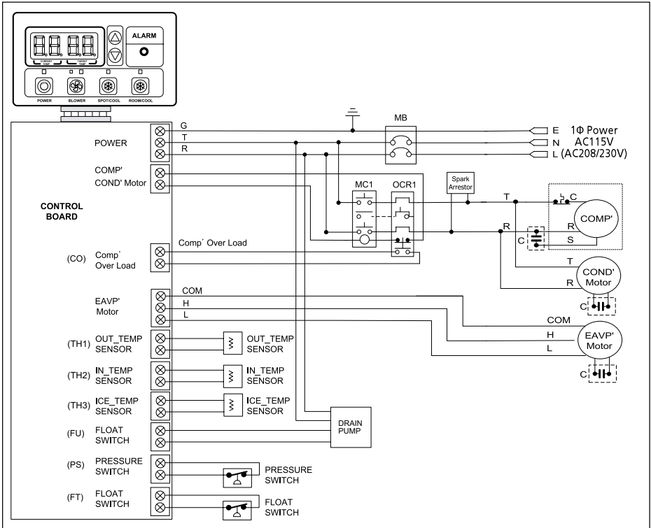
Figure 36 - Circuit Wiring Diagram (Models HPC-3000 / HPC-5000 / HPC-7000)
