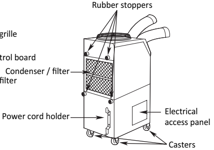
Figure 14 – Rear and Left Side View
