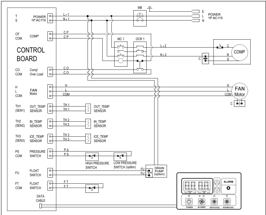
Figure 37 - Circuit Wiring Diagram (Models WPC-4000)
