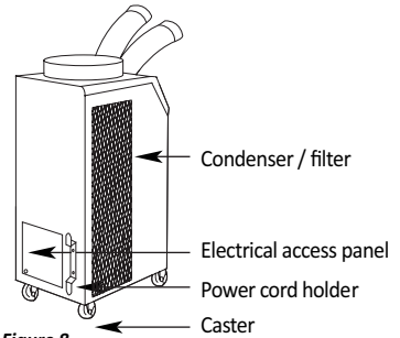
Figure 8 Back and Left Side View
