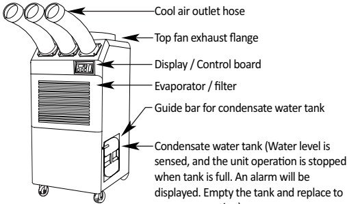
Figure 20 Front and Right Side View
