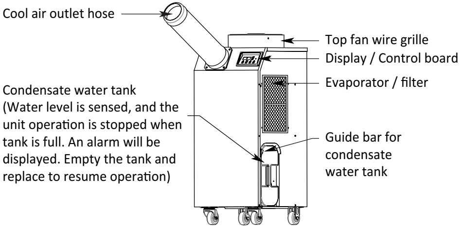
Figure 1 – Front and Right Side View
