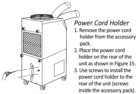
Figure 15 – Power Cord Holder attachment
