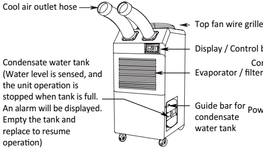
Figure 13 – Front and Right Side View
