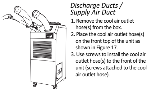
Figure 17 – Cool Air Outlet attachment
