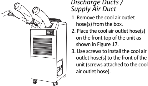
Figure 17 – Cool Air Outlet attachment
