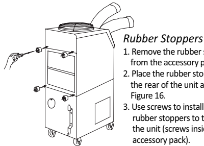
Figure 16 – Rubber Stopper attachment
